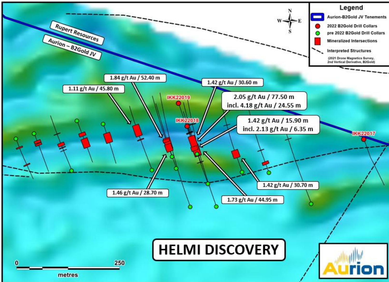
Figure 2: Drill hole locations. Aeromagnetic map as background.
