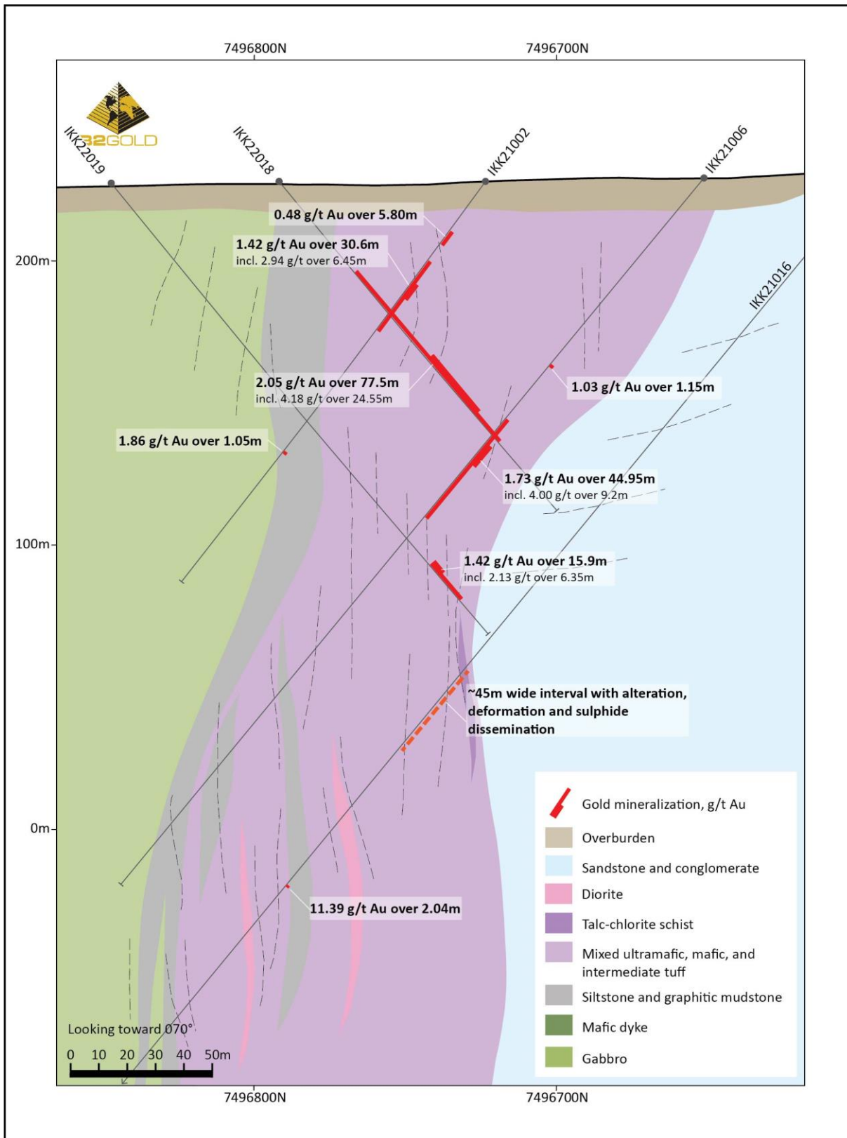
Figure 3: Cross section, holes IKK22019 and IKK22018
