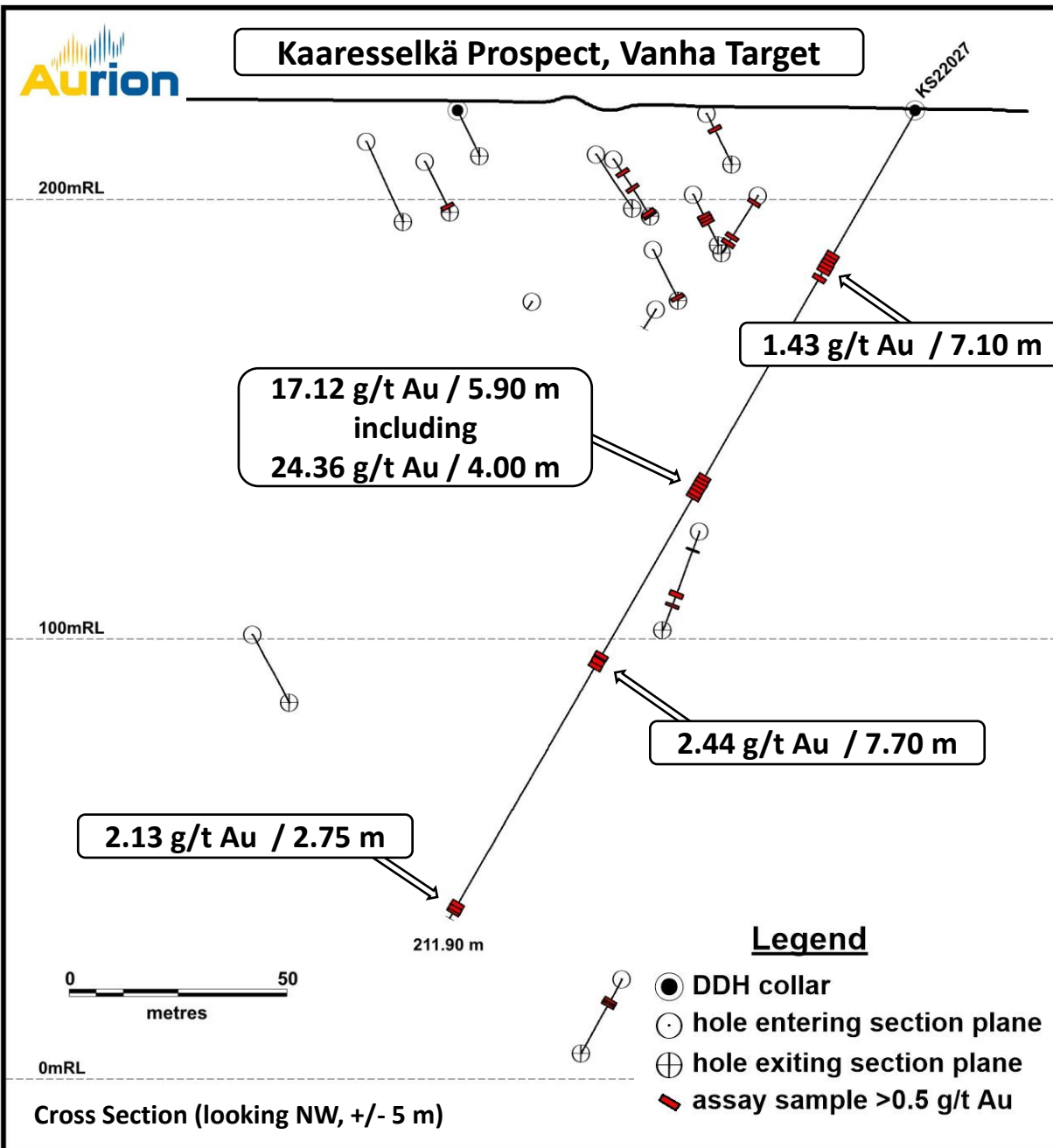
Figure 3: Cross-section along drill hole KS22027
