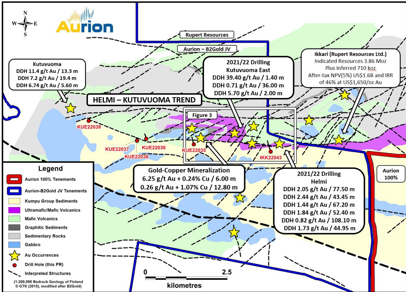
Figure 2: Map of the eastern part of the Aurion-B2Gold JV area.
