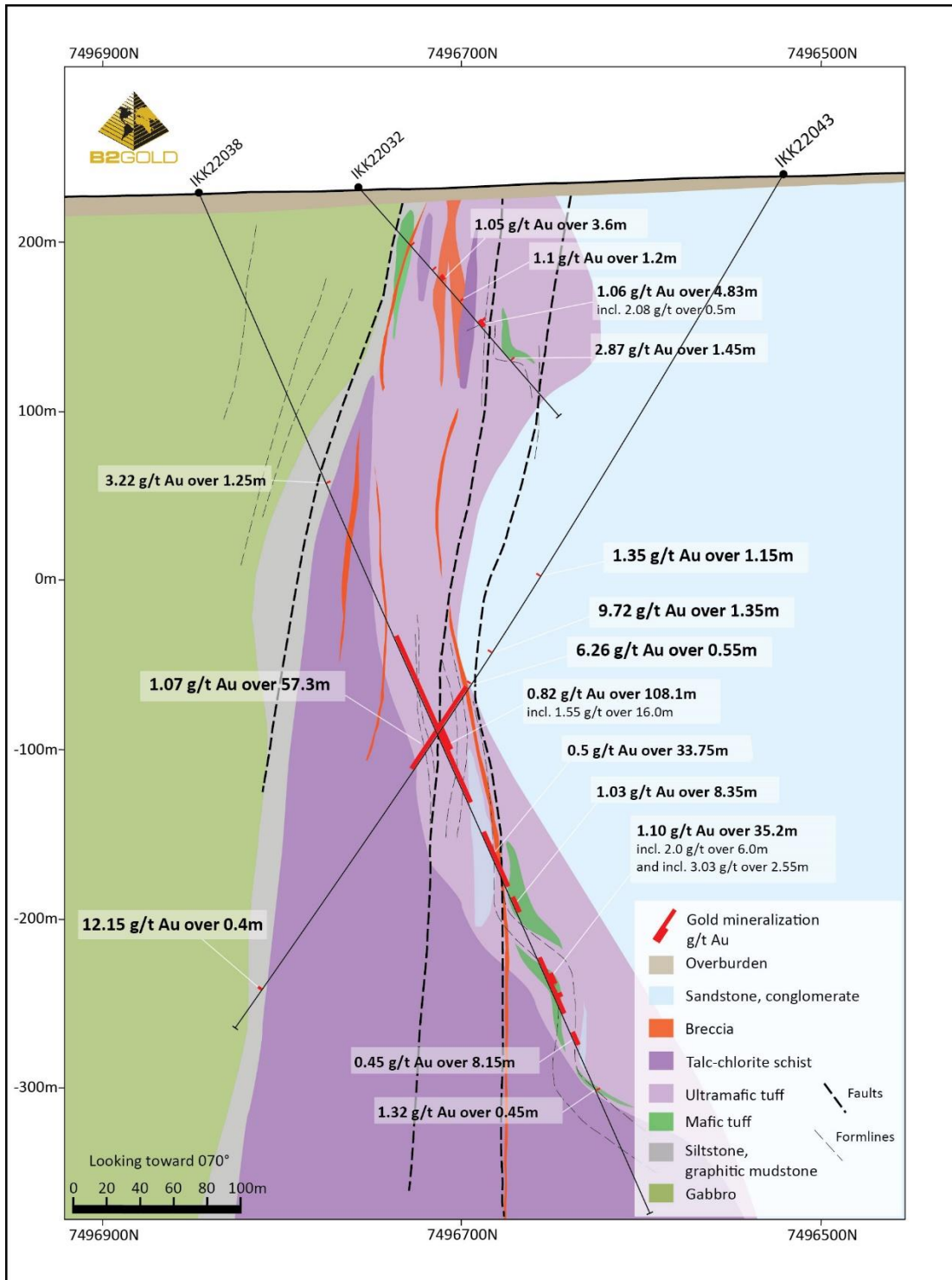
Figure 4: Cross section, holes IKK22043 and IKK22038.
