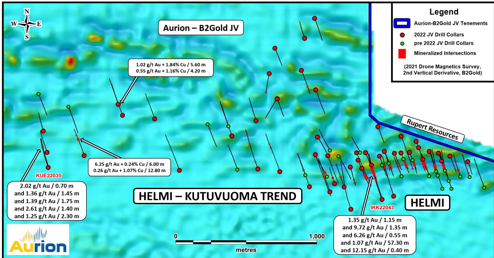
Figure 3: Drill hole locations. Aeromagnetic map as background.
