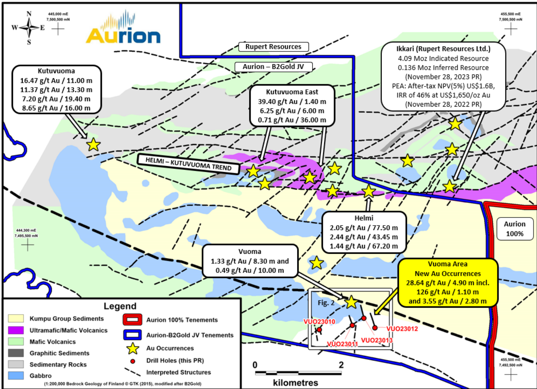
Figure 1: Map of the eastern part of the Aurion-B2Gold JV property with bedrock geology as background.
