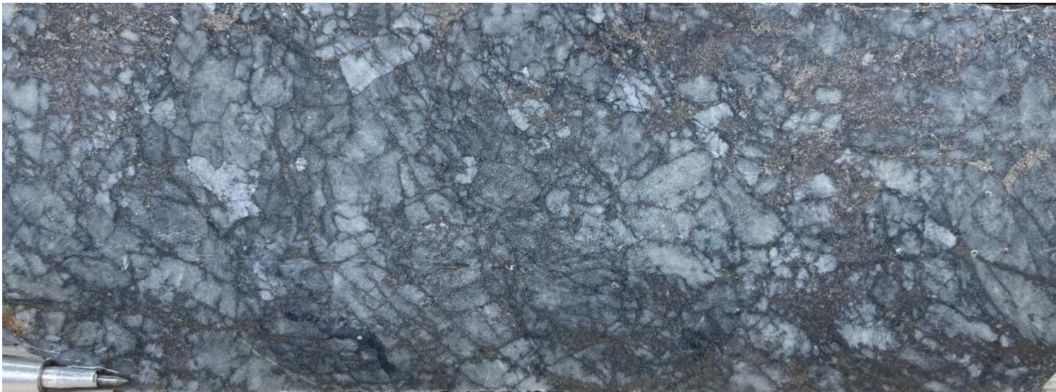
Figure 4: SOR23002: FeMg-dolomite-quartz-pyrrhotite vein breccia (2.1 g/t Au over 1.1 m from 45.7 m) part of 1.05 g/t over 40.7 m from 38.4 m.
